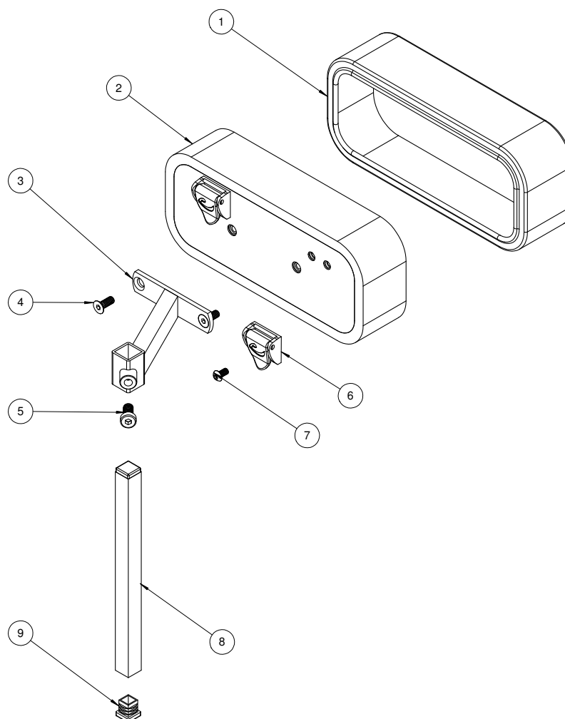
Item numbers for Backrest extension
