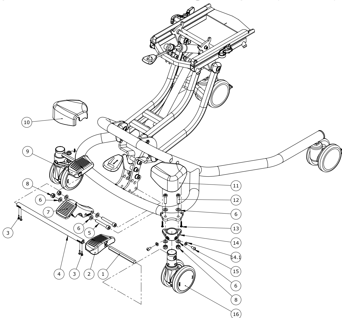
Item numbers for Foot operated central brake kit, size 2 - 3, gas and power (890012-2)
