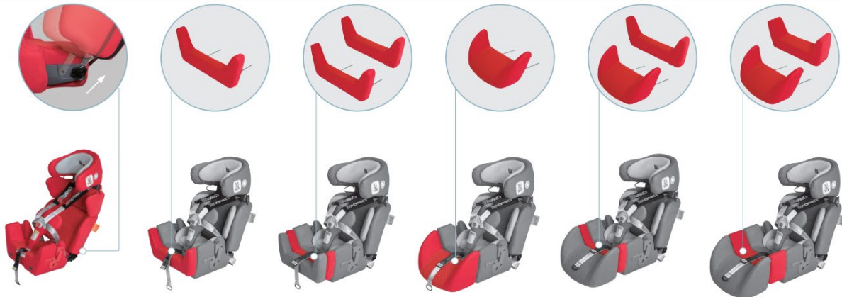
Seat Depth Adjustments 2" Rodded Seat Depth Extensions 2" Rodded + 2" Seat Depth Extensions 7" Rodded Seat Depth Extensions 7" Rodded + 2" Seat Depth Extensions 7" Rodded + 4" Seat Depth Extensions
